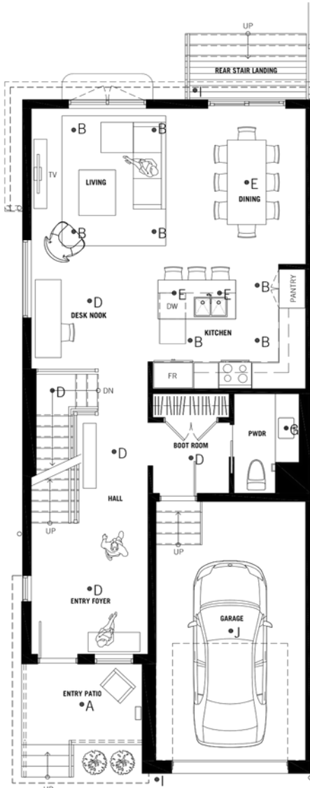
MAIN LEVEL
