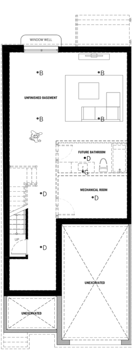
LOWER LEVEL
