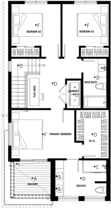
UPPER LEVEL
