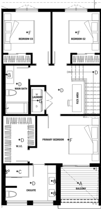
UPPER LEVEL
