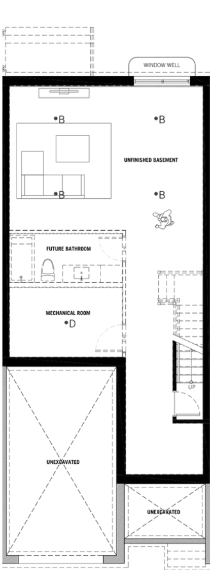
LOWER LEVEL
